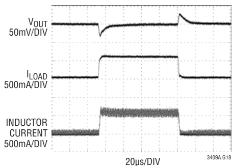
Load Step 50mA to 600mA Pulse-Skipping, V_{IN} = 3.6\text{V} , V_{OUT} = 1.8\text{V}
