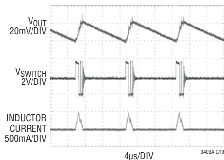
Burst Mode Operation, I_{LOAD} = 35\text{mA} , V_{IN} = 3.6\text{V} , V_{OUT} = 1.8\text{V}
